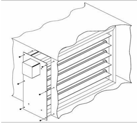
Bottom Mount:
