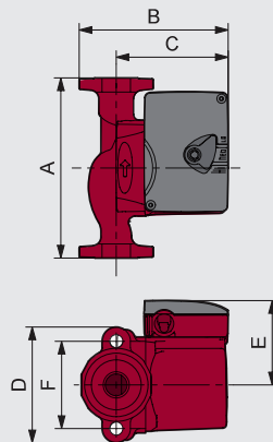
Flange FC
