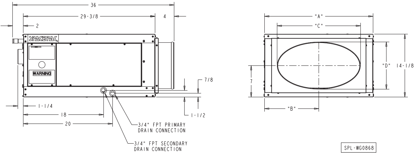
Unit Dimensions and Clearance
