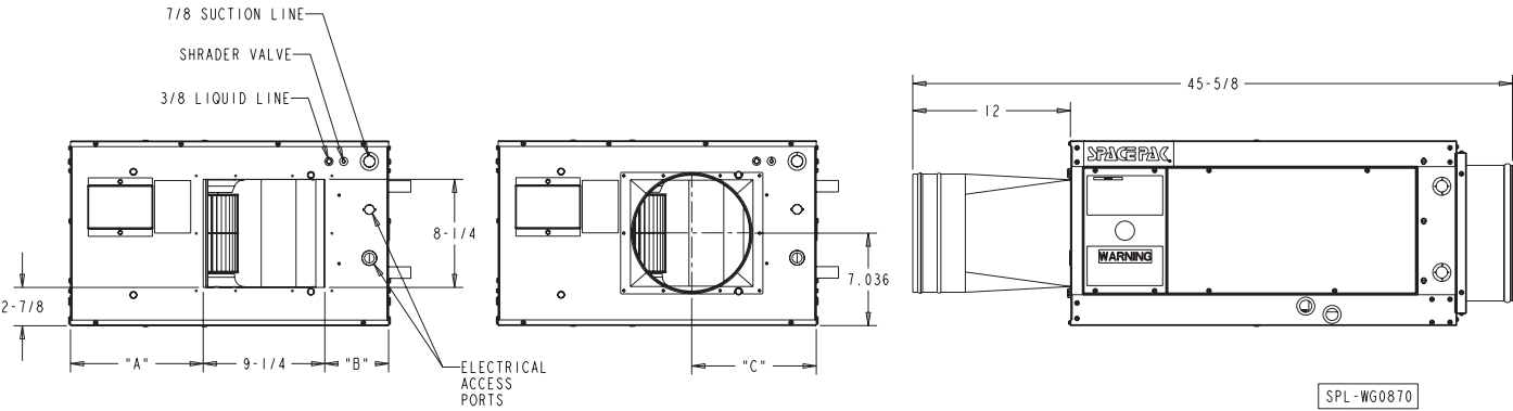
Connection Locations and Plenum Adaptor Dimensions
