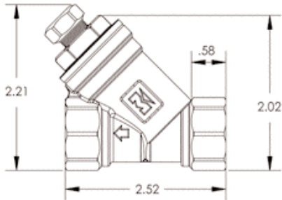
Solid Cap Option
