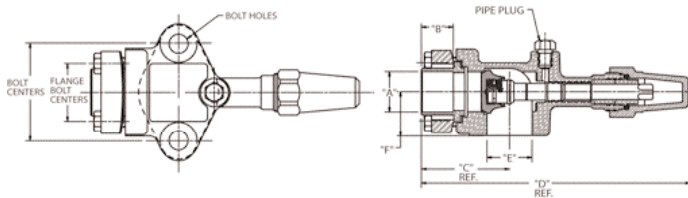
FLANGE UNION-SOLDER TYPE-PLASTIC CAP
