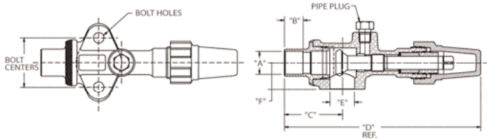
STRAIGHT PORT-SOLDER TYPE-PLASTIC CAP
