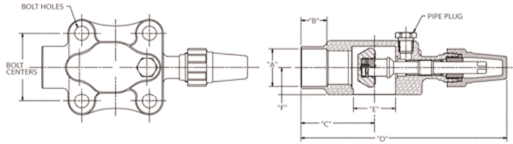
DOUBLE PORT-SOLDER TYPE-STEEL CAP
