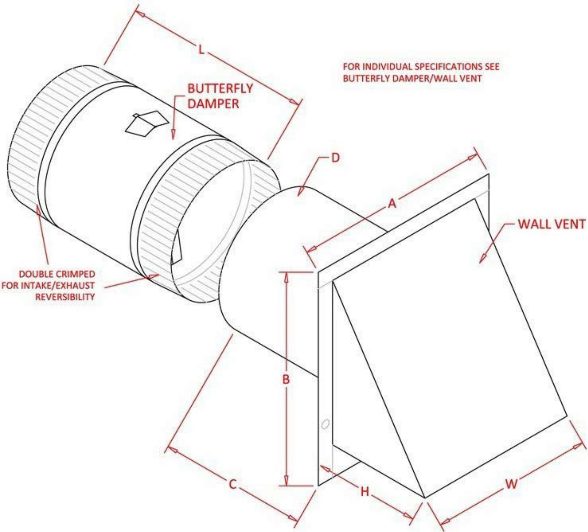
WALL VENT WITH BUTTERFLY DAMPER
