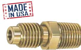
AF-13451 1/4" NPTF ACME THREAD HALF UNION
