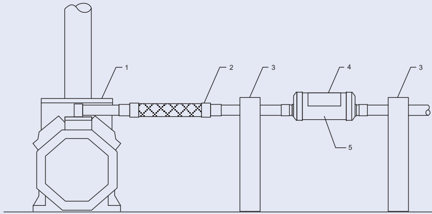
CORRECT MUFFLER SUPPORT
