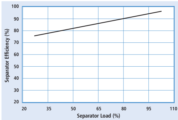
Separation Efficiency
