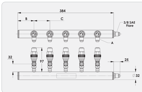
VALVE MANIFOLD
