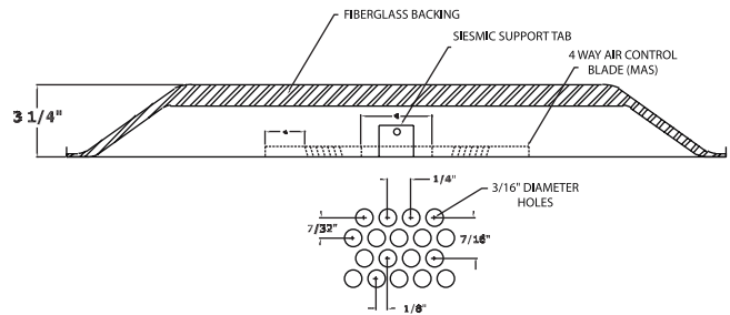
Model 1020MAS / MAR Back
