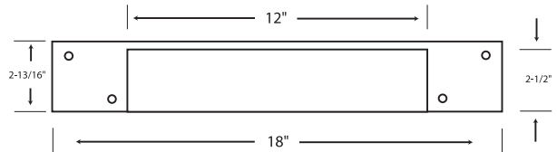
Bottom View of Model 118
