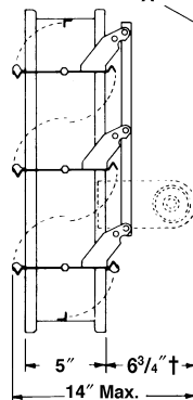
PARALLEL BLADE DEPICTED Optional Exposed Linkage.
