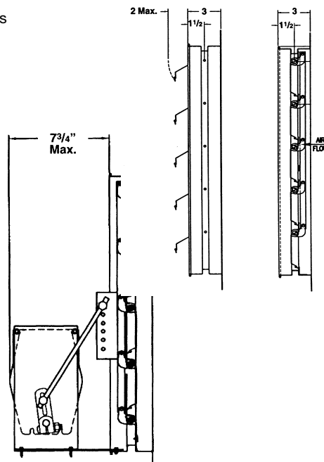
Internal Mounted Actuator
