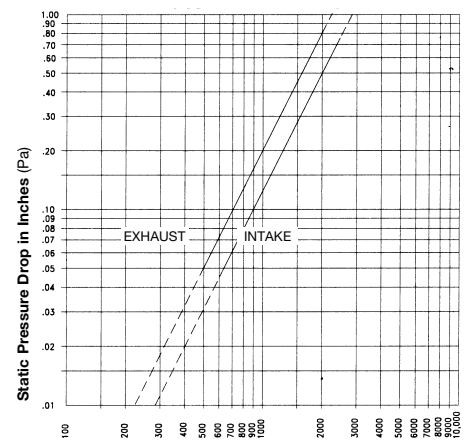
Air Velocity in feet/minute through Free Area Ratings do not include the effect of a bird screen.
