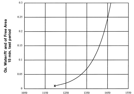
Free Area Velocity in feet per minute Standard air .075 lb/ft³
