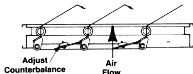
HORIZONTAL MOUNT — AIR FLOW UP
