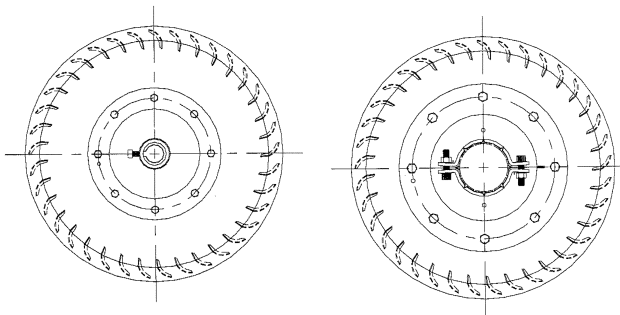
Clamplok Hub for 1/4", 3", 4", 4 1/2" and 5" Tubular Shafts
