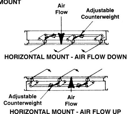
HORIZONTAL MOUNT - AIR FLOW UP
