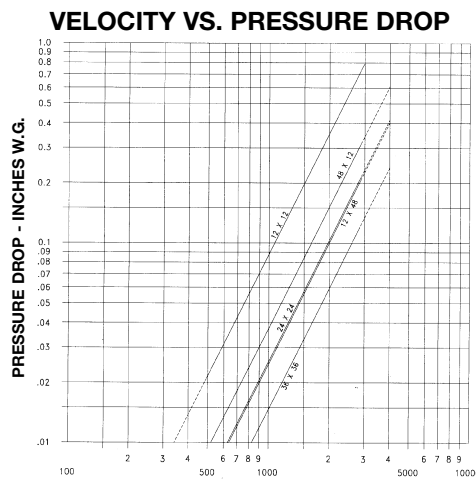
FACE VELOCITY - FEET/MINUTE — AMCA FIG. 5.3 C306 sizes 12 x 12, 24 x 24, 48 x 12, 12 x 48, 36 x 36 All data corrected to represent standard air at a density of 0.075 lbs/ft 3 .
