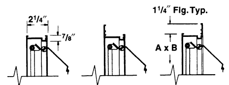
FRAME CONSTRUCTIONS
