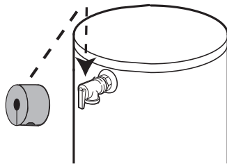
Typical Side Connect T & P Arrangement.
