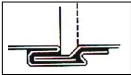
Snaplock Seam
