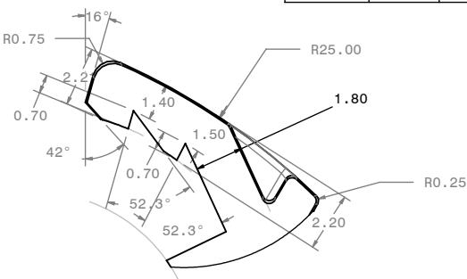
DETAIL D SCALE 4 : 1
