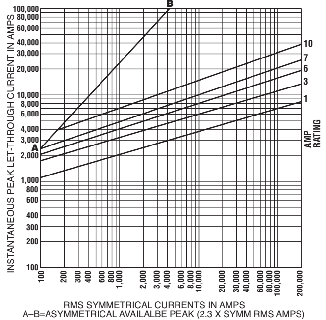
Cat. No. JDL (Amp)
