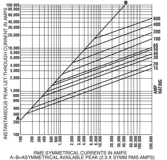
RMS SYMMETRICAL CURRENTS IN AMPS A-B=ASYMMETRICAL AVAILABLE PEAK (2.3 X SYMM RMS AMPS)
