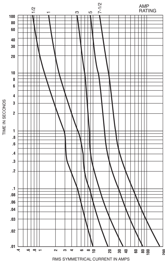
Cat. No. HCTR (Amp) Time-Delay
