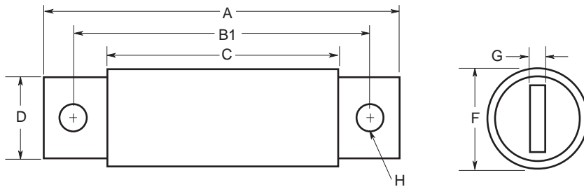
Figure 1: 4 – 30A & 225 – 1000A Range
