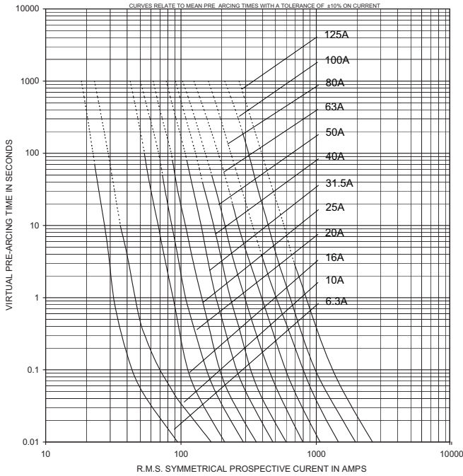
FUSE TYPES: TDL/THL/TKL TIME- CURRENT CHARACTERISTIC FOR 12KV FUSE-LINKS
