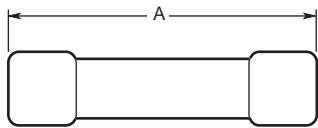
Ferrule Design—1 through 60A
