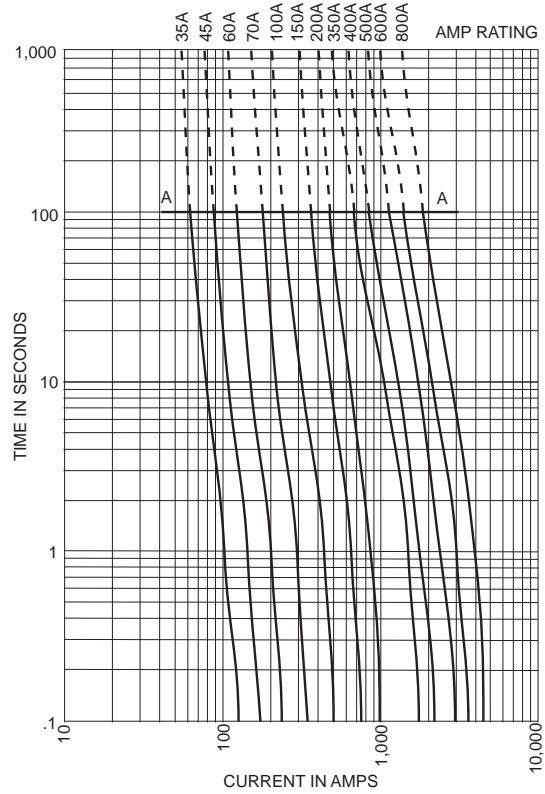
E25S(Amp) High Speed Fuse 35 – 800A, 250V
