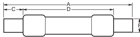
Knife Blade—70 through 600A
