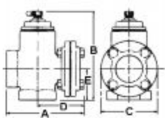
SIZES 2" AND ABOVE STRAIGHT-ANGLE VALVES
