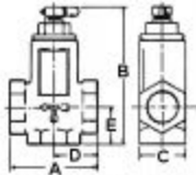
SIZES 3/4" - 1" - 1 1/4" - 1 1/2" STRAIGHT-ANGLE VALVES
