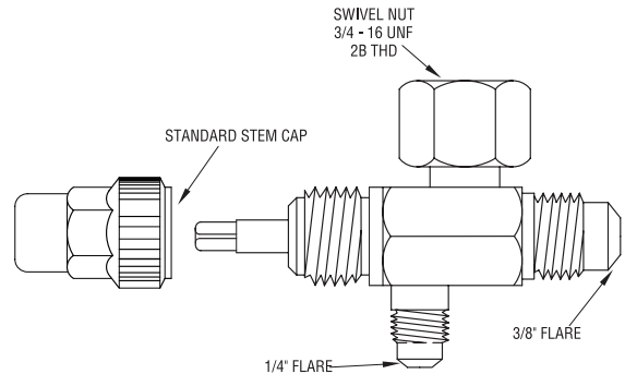
Rotalock Valve
