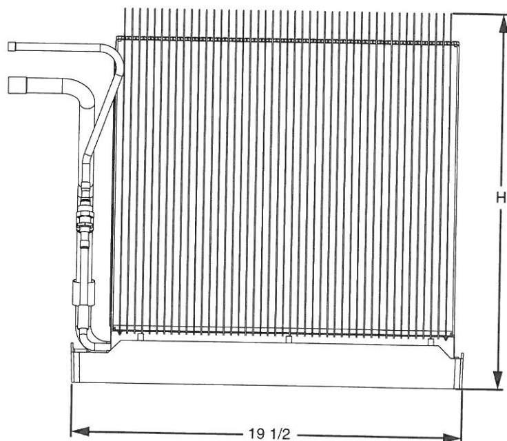
Uncased Coil
