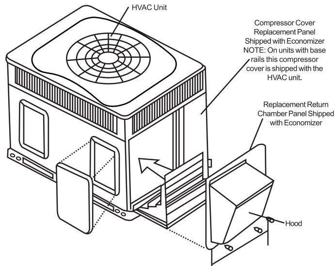
Vertical Economizer
