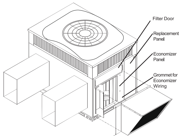
Horizontal Economizer
