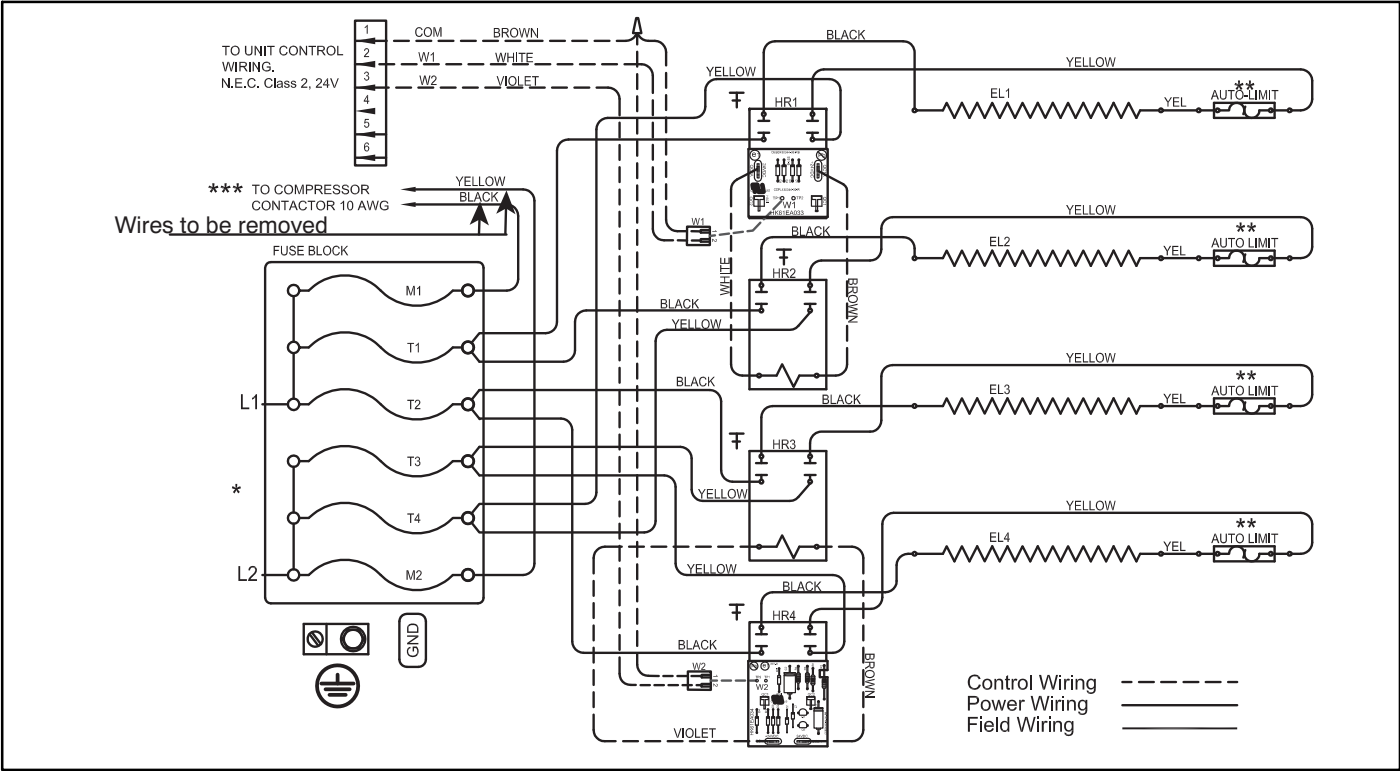
NOTE: 20 kW shown. Smaller heaters have fewer elements and controls. Single-Phase Accessory Electric Heater Wiring
