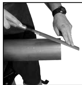
Figure 4: Deburr outside diameter using a half-round file
