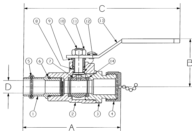
PC585-70-66-HC P x Hose
