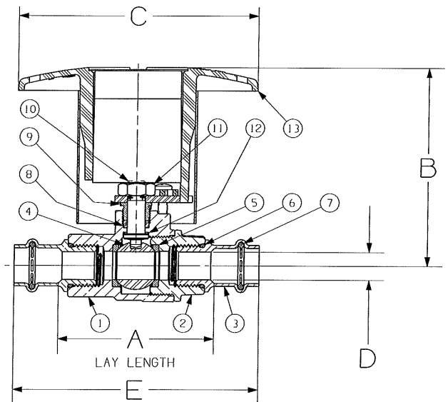
PC585-70-NS P x P
