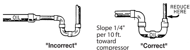
Figure 9. Suction P-Traps
