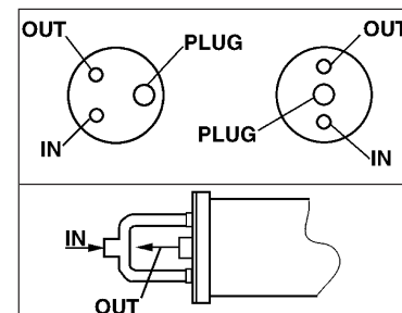
Figure 5. Water Connections
