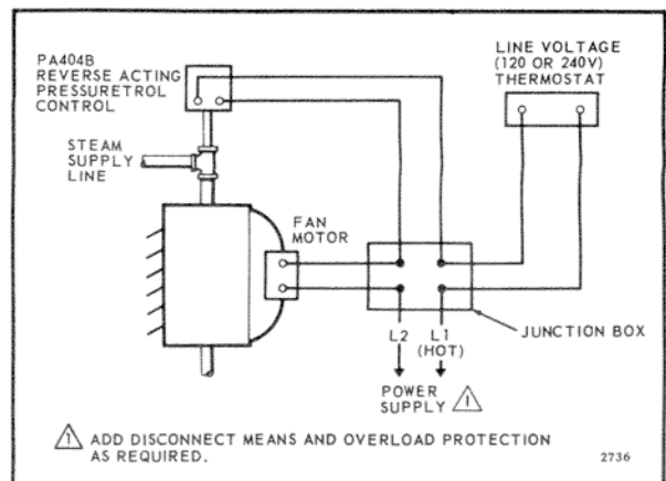
FIG. 5—TYPICAL CONNECTIONS FOR A PA404B USED IN A UNIT HEATER INSTALLATION.
