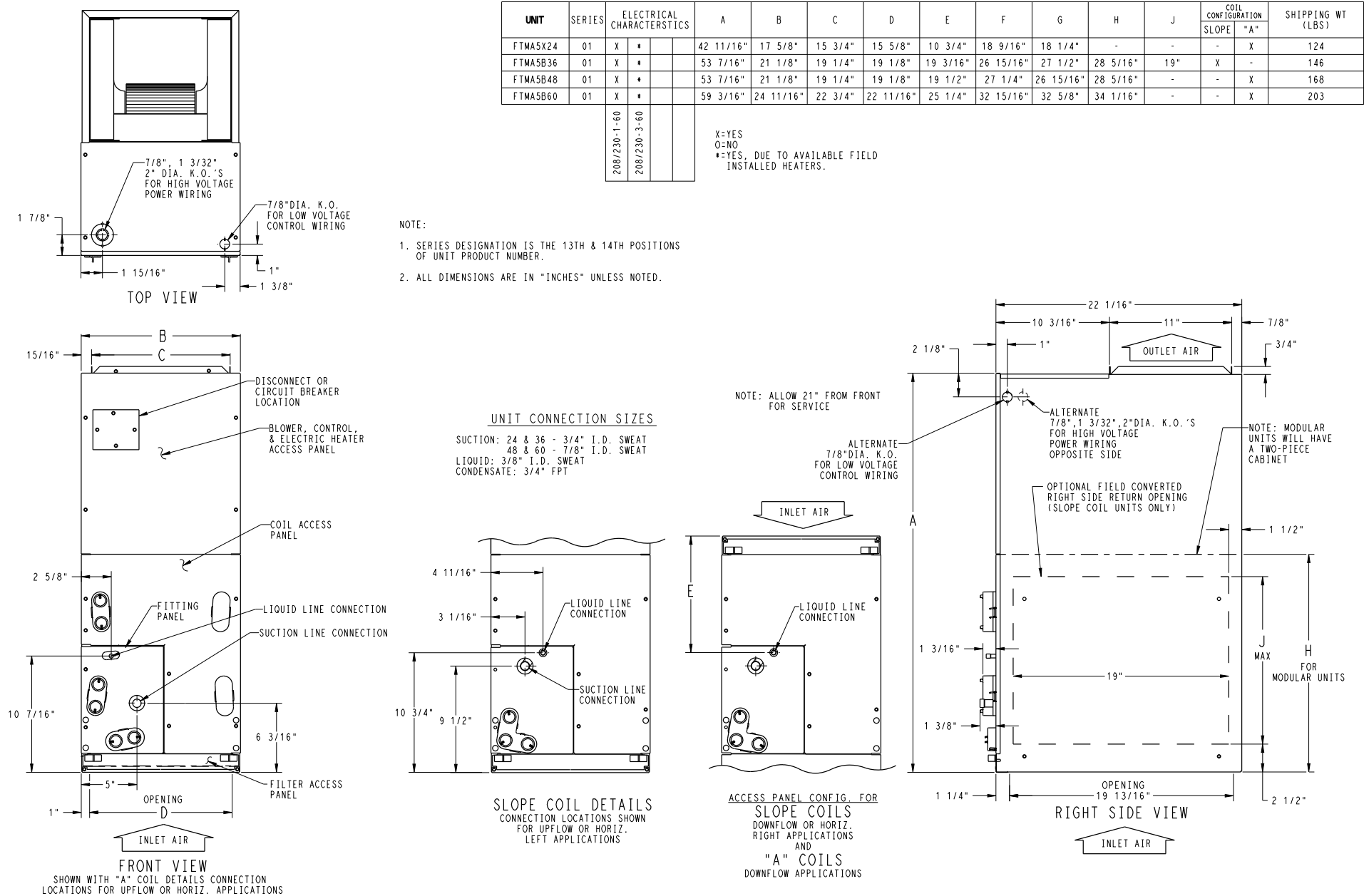
Fig. 1 – Dimensions, sheet 1
