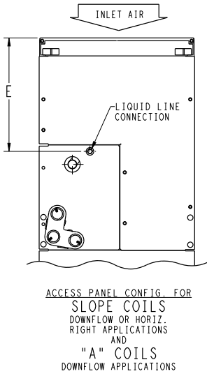
Fig. 3 – Dimensions, sheet 3
