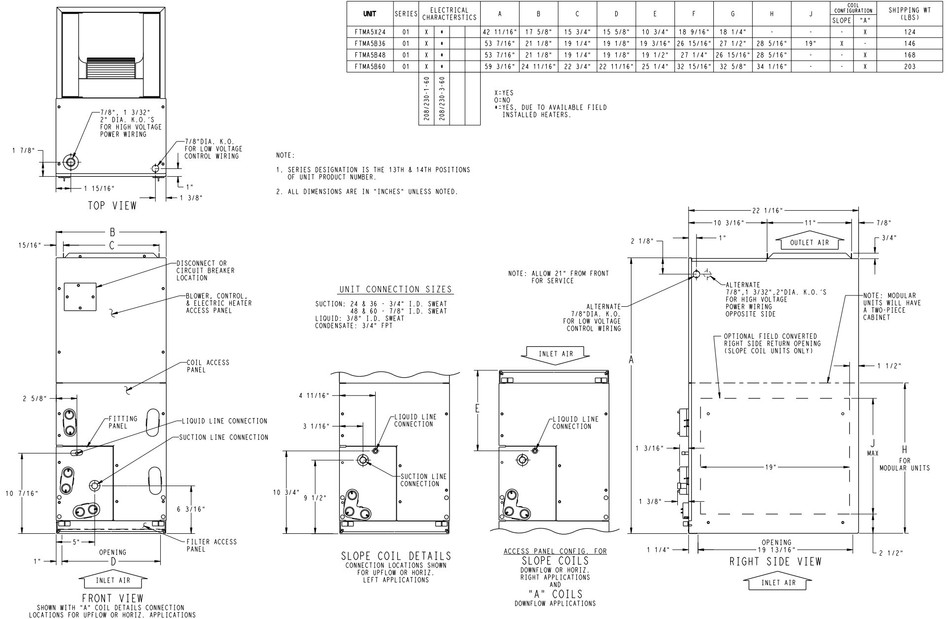
Fig. 1 – Dimensions, sheet 1
