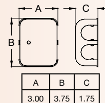
X101 Junction Box (16)
