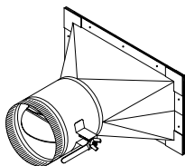
3400-DS TAKEOFF CENTER TAPER with 2" DAMPER HANDLE STANDOFF (4" - 12")
