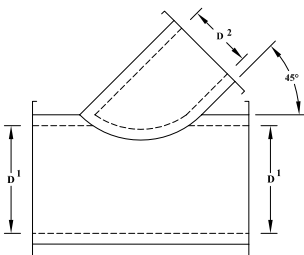
DW6276 45° LATERAL
