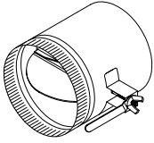
175-XS1 DAMPER SLEEVE 2" DAMPER HANDLE STANDOFF (SIZES 4" - 12")
