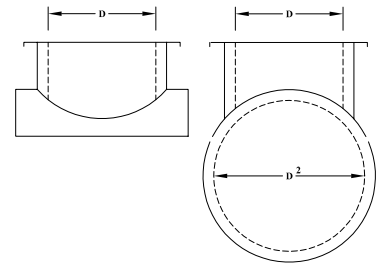
DW6307 SADDLE TAP
