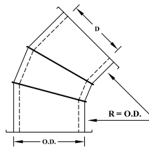
DW6121 45° ELBOW 3 Piece Gorelock
