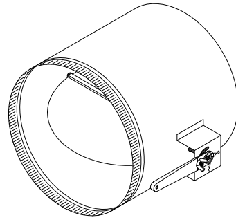
175-XS2 DAMPER SLEEVE with \frac{3}{8} " SOLID ROD AXIS & 2" STANDOFF (14" - 20")
