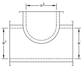
DW6271 90° TEE
