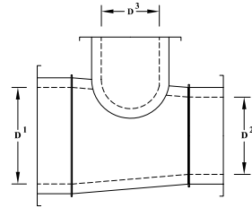
DW6271R REDUCING 90° TEE
