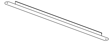
1254 MOUNTING BRACKET Screw-on bracket for use with unflanged Boots and Boxes 25" long, 26 ga. Galvanized
