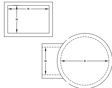
DW6406 GRILLE TAP
