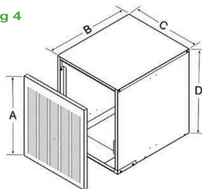
UPFLOW/DOWNFLOW COIL BOX CABINET DIMENSIONS (FIG 4)
