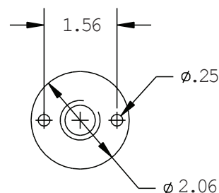
MOUNTING
