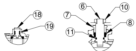
STEM DETAIL
