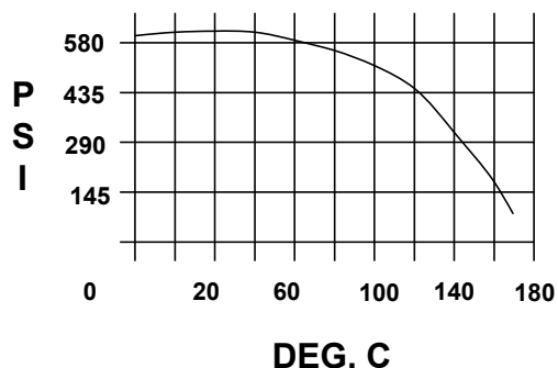
PRESS. VS. TEMP. CURVE
