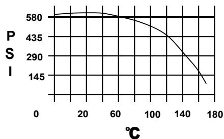
PRESS. VS. TEMP. CURVE
