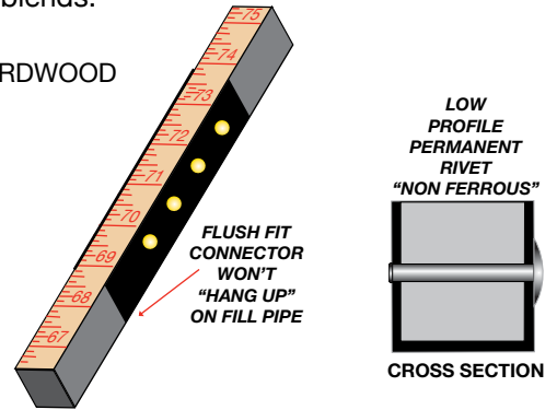
HEAVY DUTY ALUMINUM CONNECTOR "NON FERROUS"
