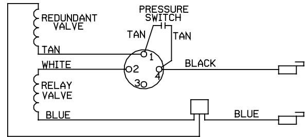
WIRING DIAGRAM
