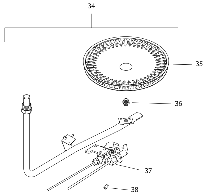
LP GAS (SX) BURNER ASSEMBLY
