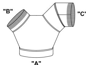
278 1-WAY ADJUSTABLE WYE
