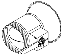
3200-DS2 CONICAL SPIN-IN with 3/8" SOLID ROD AXIS & 2" STANDOFF (4" - 12")
