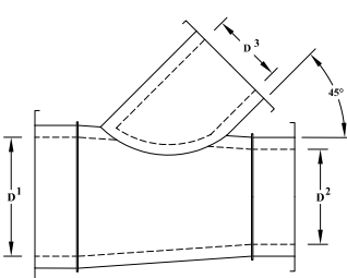
DW6276R REDUCING 45° LATERAL
