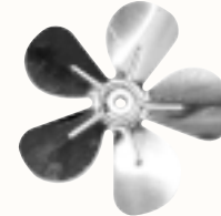
No. 26-104 CW 5 1/2 in. Aluminum fan blade, shaft mounted 1/4 in. w/set screw.
